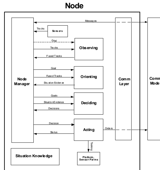
Figure 4 Internal OODA Structure of a Node.
