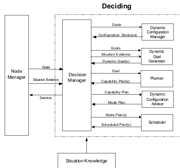
Figure 7 Deciding Module
