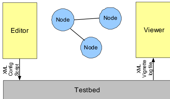
Figure 2 High-Level Testbed Architecture
